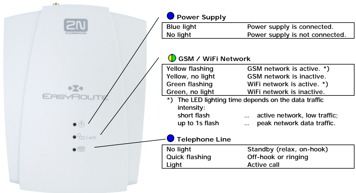
Figure 2.1 2N ® EasyRoute LED Indicators
